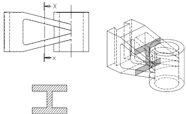
Figure 1-17 Removed Section
