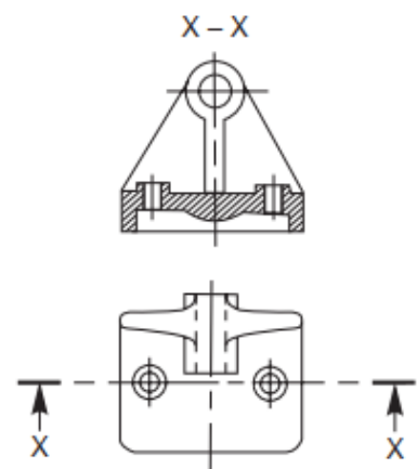
Figure 1-11 Sectioning
