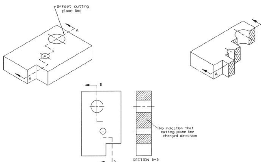
Figure 1-14 Offset Sections
