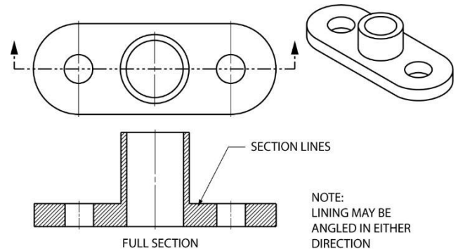
Figure 1-12 Full Sections
