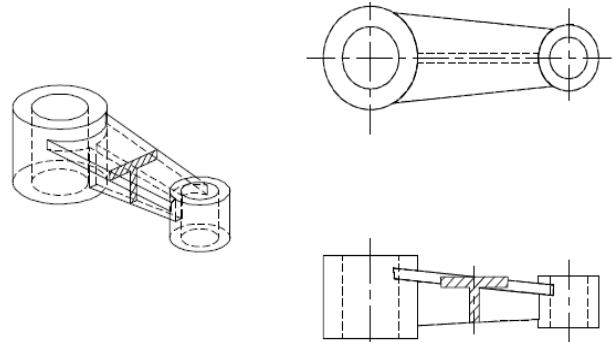
Figure 1-16 Revolved Section
