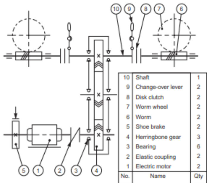
Figure 2-5 Schematic assembly drawing
