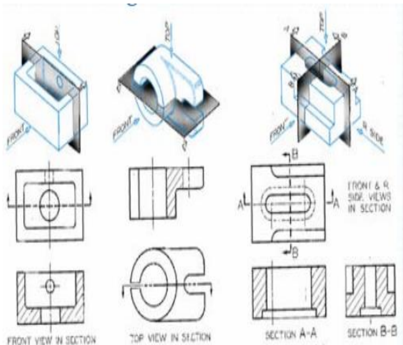
Figure 1-21 Example of hatching
