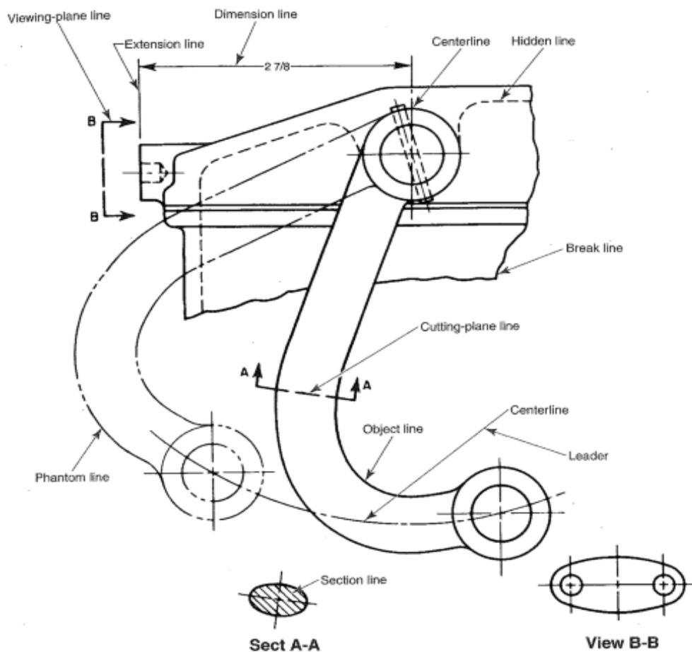
Figure 1-5 Standard line types and line weights B
