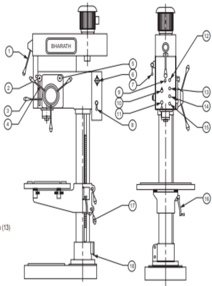
Figure 2-3 Assembly drawing for instruction manual
