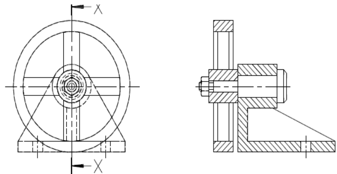
Figure 1-18 Parts not sectioned
