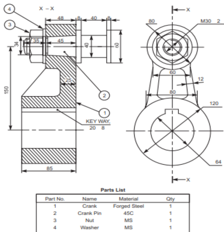
Figure 2-1 Assembly Drawing
