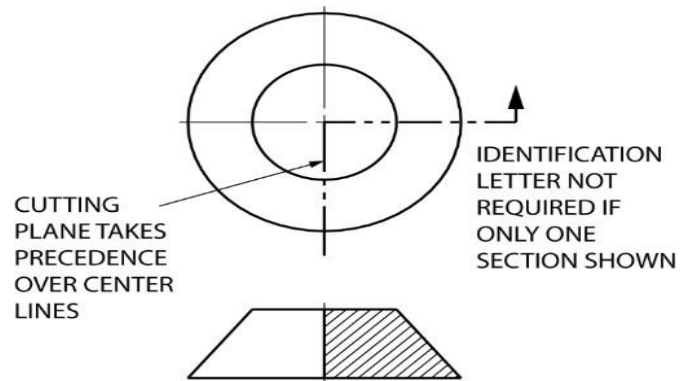
Figure 1-13 Half Sections
